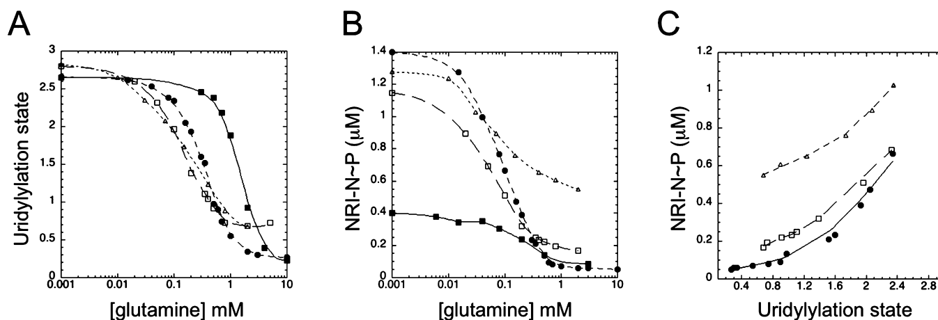
Figure 6. Comparison of bicyclic systems where the PII/NRII ratio was varied 25-fold. (A) Regulation of PII uridylation state by glutamine. \triangle , PII was 0.1 \mu\text{M} , NRII was 0.5 \mu\text{M} , and the sensitivity corresponded to n_H \sim 1.11 ; \square , PII and NRII were both 0.1 \mu\text{M} , and the sensitivity corresponded to n_H \sim 1.36 ; \bullet , PII was 0.5 \mu\text{M} and NRII was 0.1 \mu\text{M} , and the sensitivity corresponded to n_H \sim 1.55 ; \blacksquare , reference sample where PII was 5 \mu\text{M} and NRII was 0.1 \mu\text{M} , and the sensitivity corresponded to n_H \sim 2.13 . (B) Regulation of NRI phosphorylation state by glutamine. Symbols are as in panel A, sensitivities were as follows: \triangle , 1.19; \square , 1.26; \bullet , 1.34; \blacksquare , 1.06. (C) Relationship between the modification states of PII and NRI for the three systems where the NRII/PII ratio was varied 25-fold. For panels A and B, values plotted on the Y axis were obtained in the absence of glutamine.
