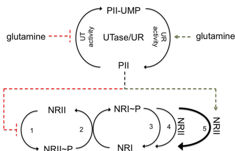
Figure 1. Activities of the UTase/UR-P-II-NR-II-NRI bicyclic signal transduction system. The UTase/UR-P-II cycle brings about the interconversion of PII and PII-UMP. The UT activity of UTase/UR catalyzes the uridylylation of PII and is inhibited by glutamine. The UR activity of the UTase/UR catalyzes the deuridylylation of PII-UMP and is stimulated by glutamine. PII regulates the phosphorylation state of NRI indirectly, by interacting with NR-II: 1, autophosphorylation activity of NR-II, which is inhibited by PII; 2, phosphotransfer activity in which phosphoryl groups are transferred from NR-II~P to NRI; 3, autophosphatase activity of NRI~P, in which it catalyzes its own dephosphorylation; 4, basal “phosphatase activity” of NR-II, in which it brings about dephosphorylation of NRI~P; 5, PII-stimulated “phosphatase” activity of NR-II. Note that steps 4 and 5 may reflect stimulation of the NRI~P autophosphatase activity by NR-II acting alone (step 4) or by NR-II in complex with PII (step 5).
